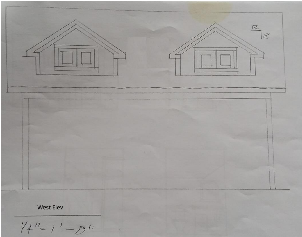
West Elevation
