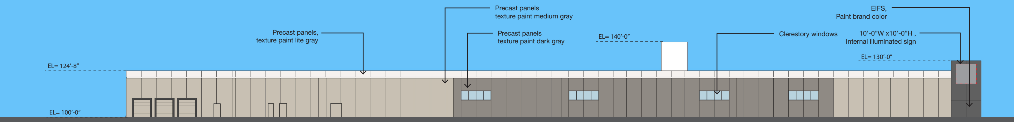
NORTH ELEVATION
