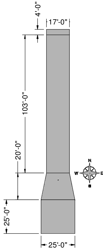
PLAN VIEW OF PLANT
