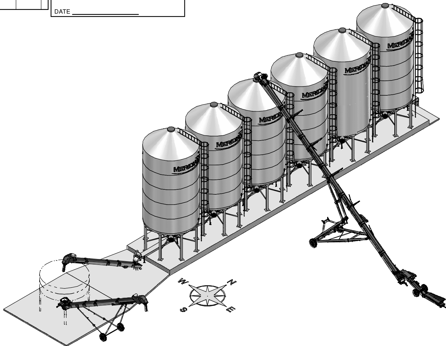
ISOMETRIC VIEW OF PLANT
