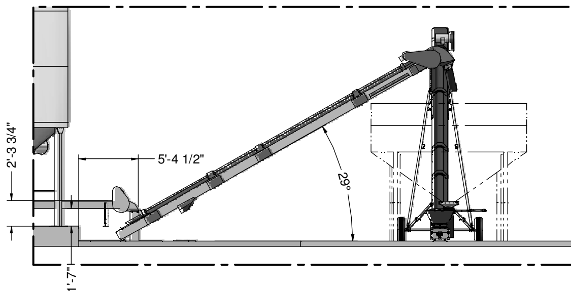
ELEVATION A OF PLANT
