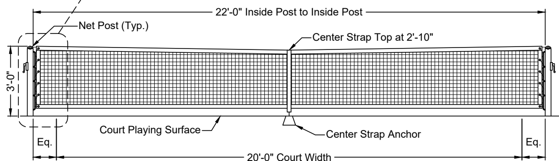
Pickleball Net Elevations Scale: None
