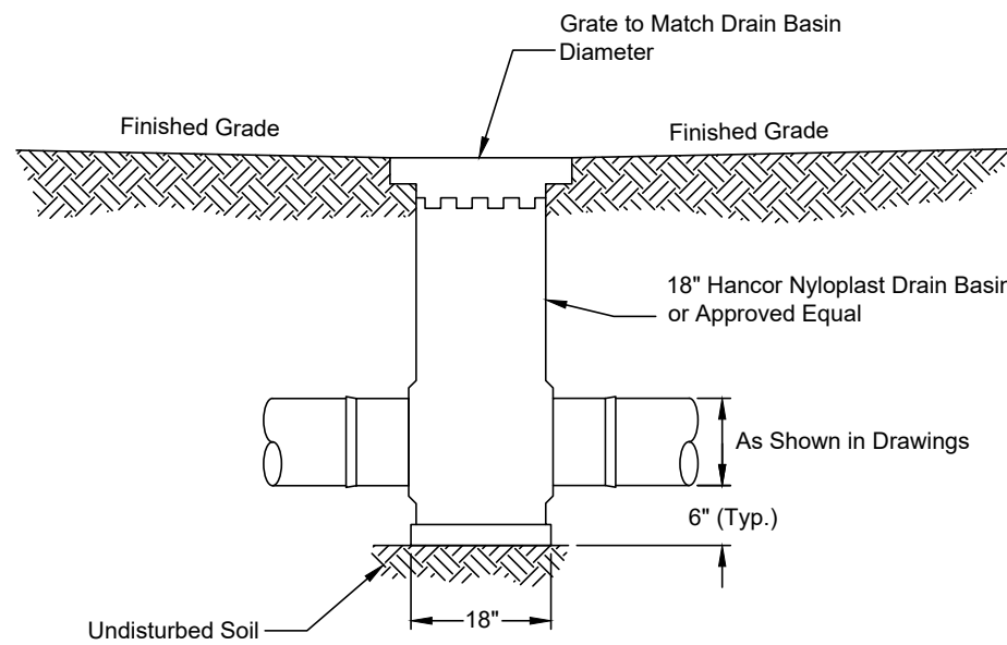
18" Drain Basin Scale: None
