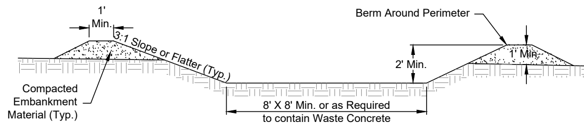
Cross Sectional View Concrete Washout Facility
