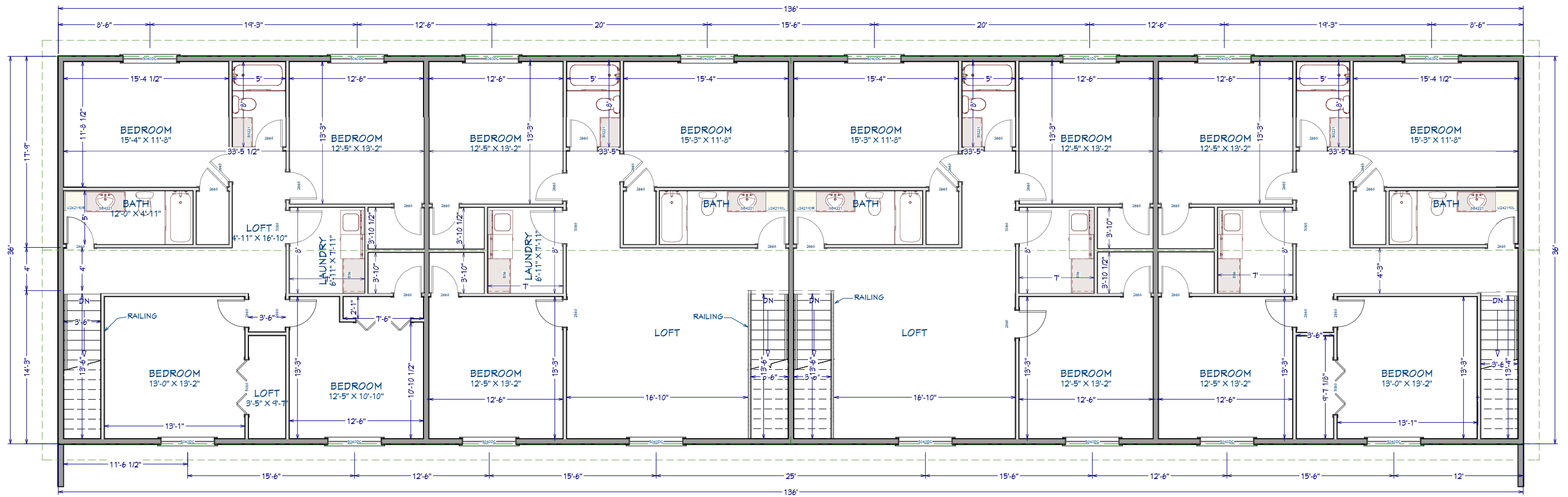
2nd Floor
