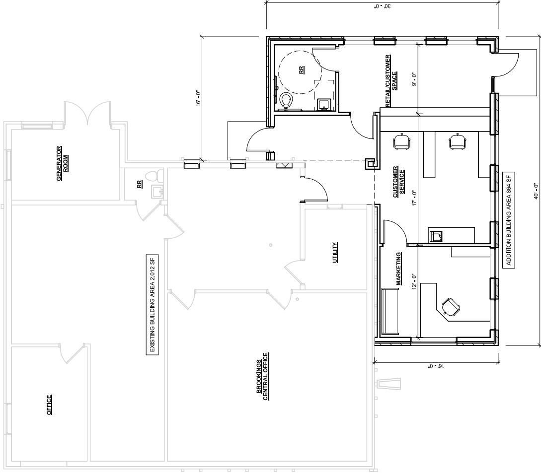
MAIN FLOOR PLAN 1/8" = 1'-0" NORTH
