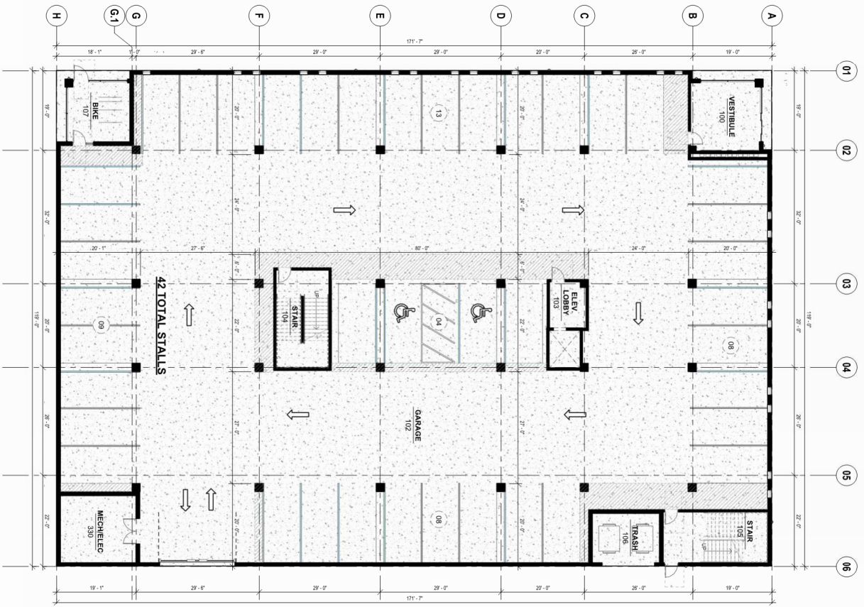
1 FIRST FLOOR PLAN 1" = 16'-0"
